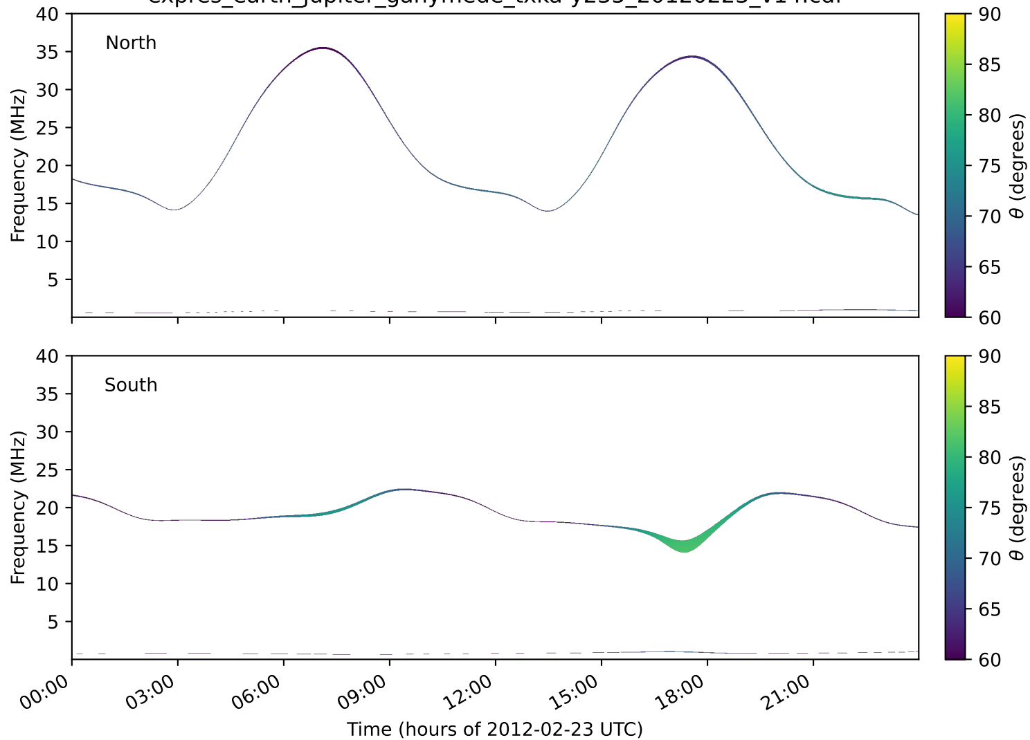
expres_earth_jupiter_ganymede_txka-y235_20120223_v14.cdf
