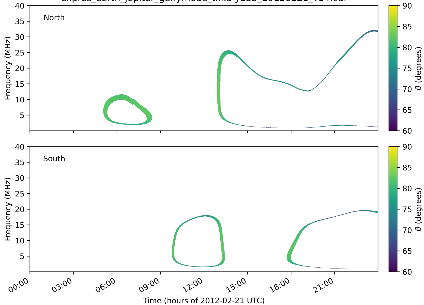
expres_earth_jupiter_ganymede_txka-y235_20120221_v14.cdf
