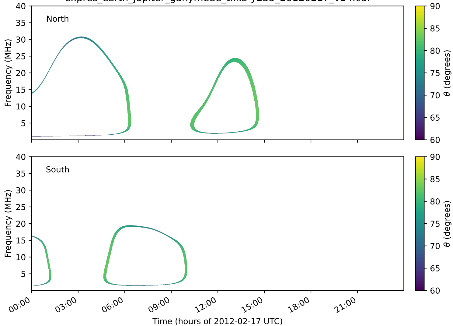
expres_earth_jupiter_ganymede_txka-y235_20120217_v14.cdf
