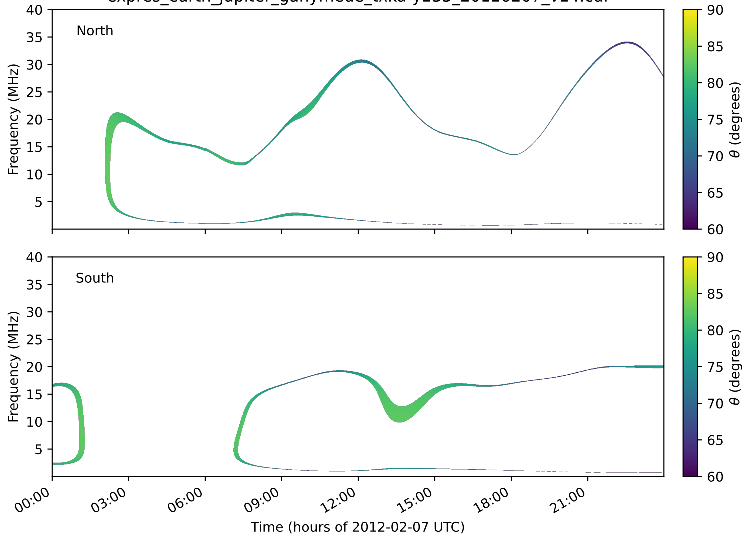
expres_earth_jupiter_ganymede_txka-y235_20120207_v14.cdf
