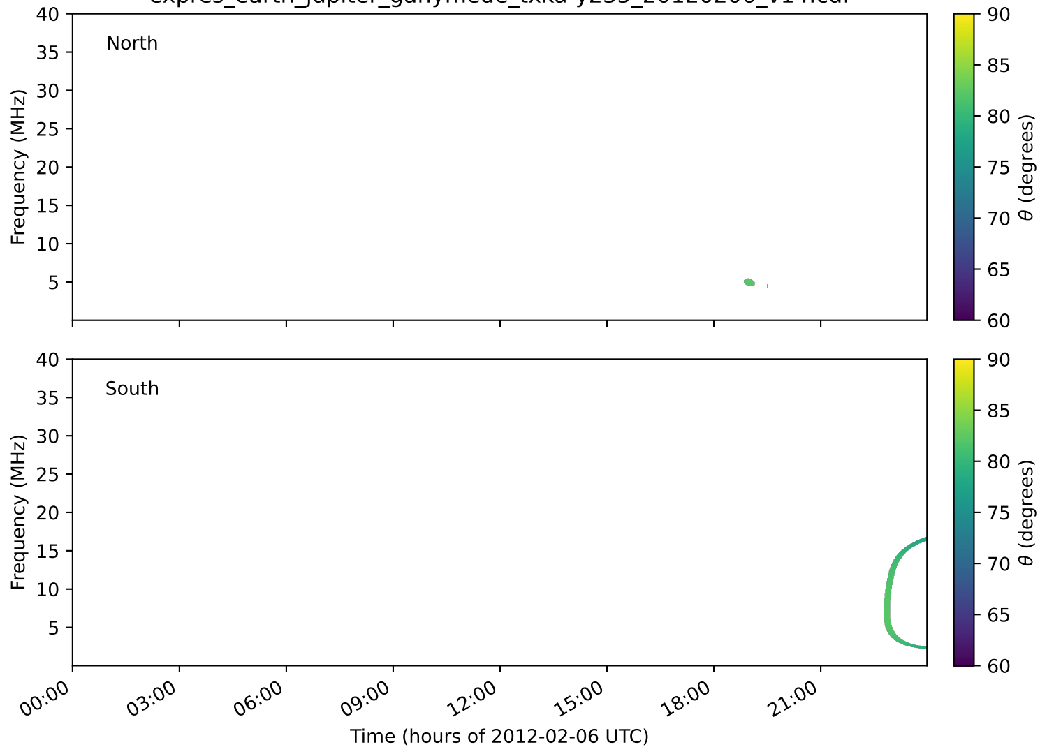
expres_earth_jupiter_ganymede_txka-y235_20120206_v14.cdf
