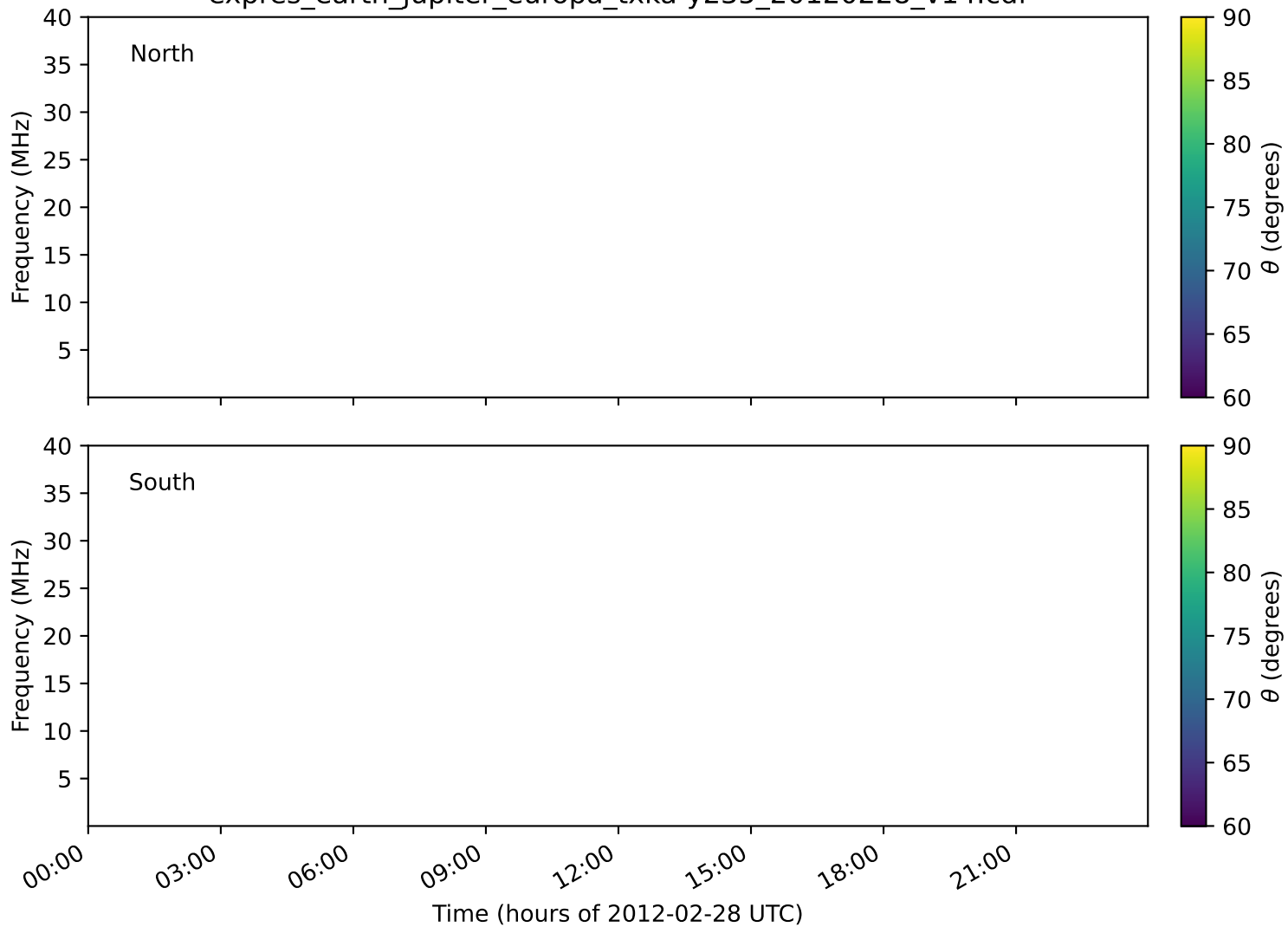
expres_earth_jupiter_europa_txka-y235_20120228_v14.cdf
