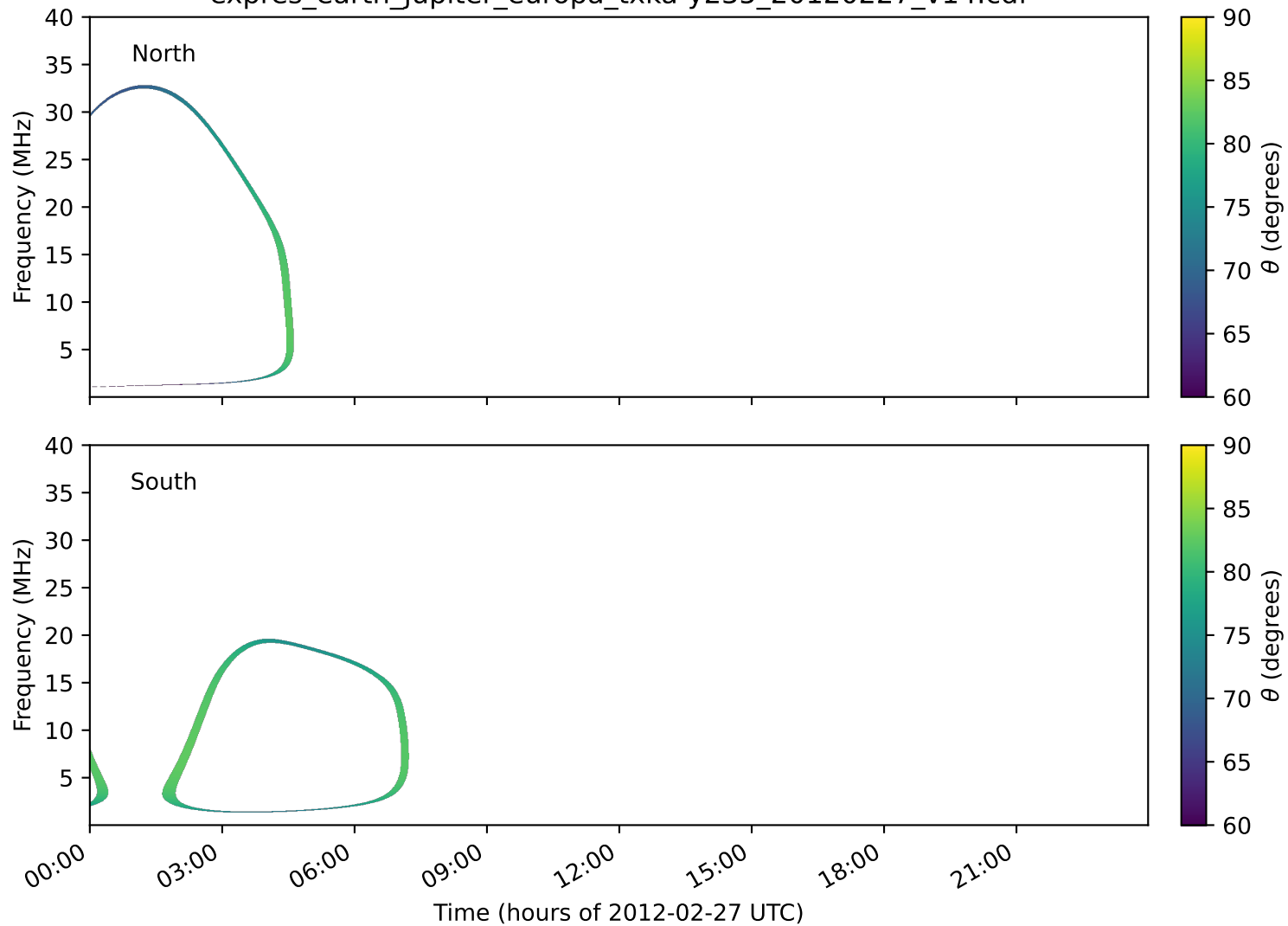
expres_earth_jupiter_europa_txka-y235_20120227_v14.cdf
