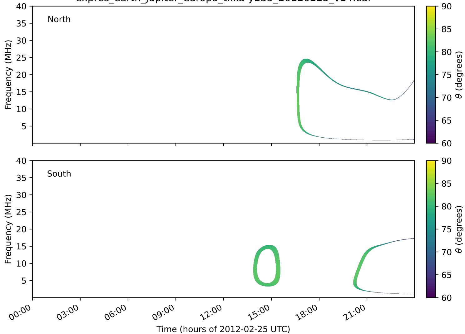
expres_earth_jupiter_europa_txka-y235_20120225_v14.cdf
