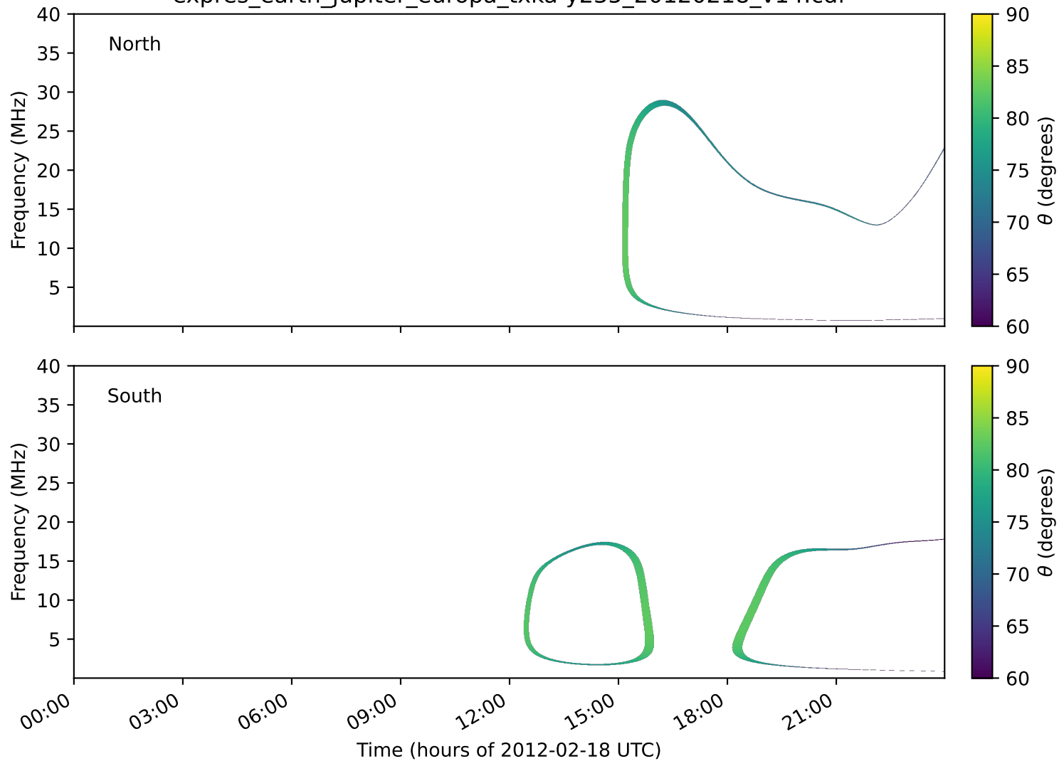
expres_earth_jupiter_europa_txka-y235_20120218_v14.cdf
