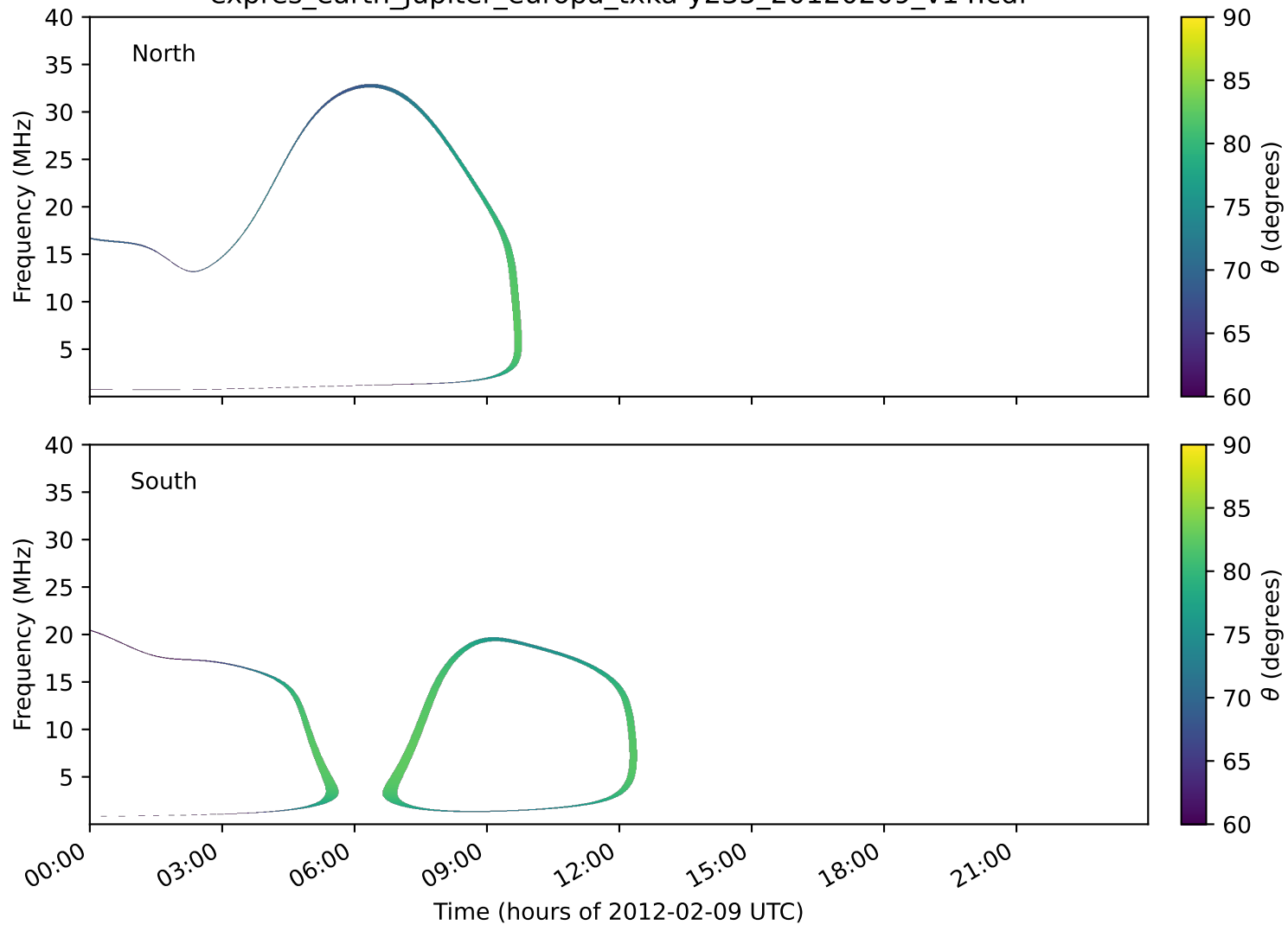
expres_earth_jupiter_europa_txka-y235_20120209_v14.cdf
