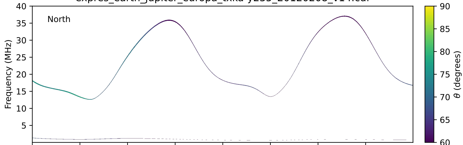
expres_earth_jupiter_europa_txka-y235_20120208_v14.cdf
