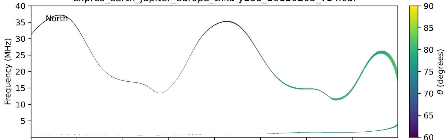
expres_earth_jupiter_europa_txka-y235_20120205_v14.cdf
