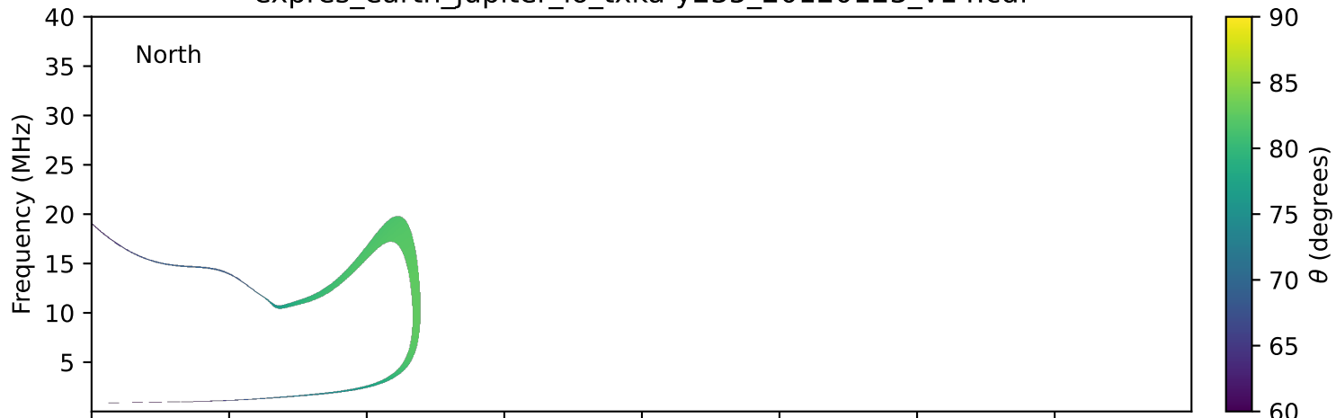
expres_earth_jupiter_io_txka-y235_20120123_v14.cdf
