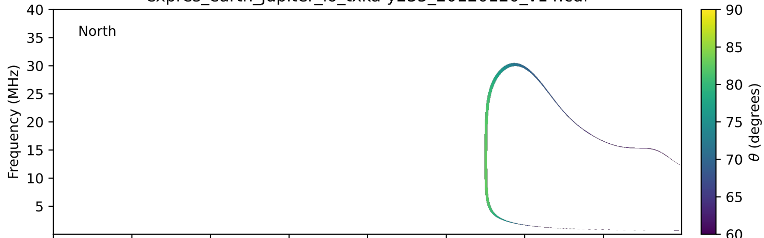
expres_earth_jupiter_io_txka-y235_20120120_v14.cdf
