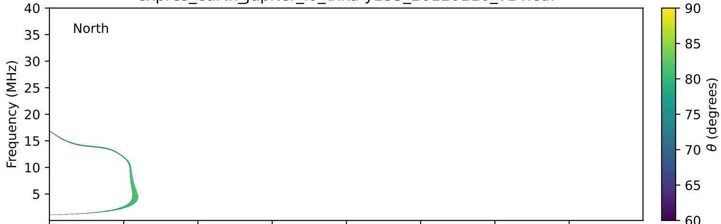
expres_earth_jupiter_io_txka-y235_20120116_v14.cdf
