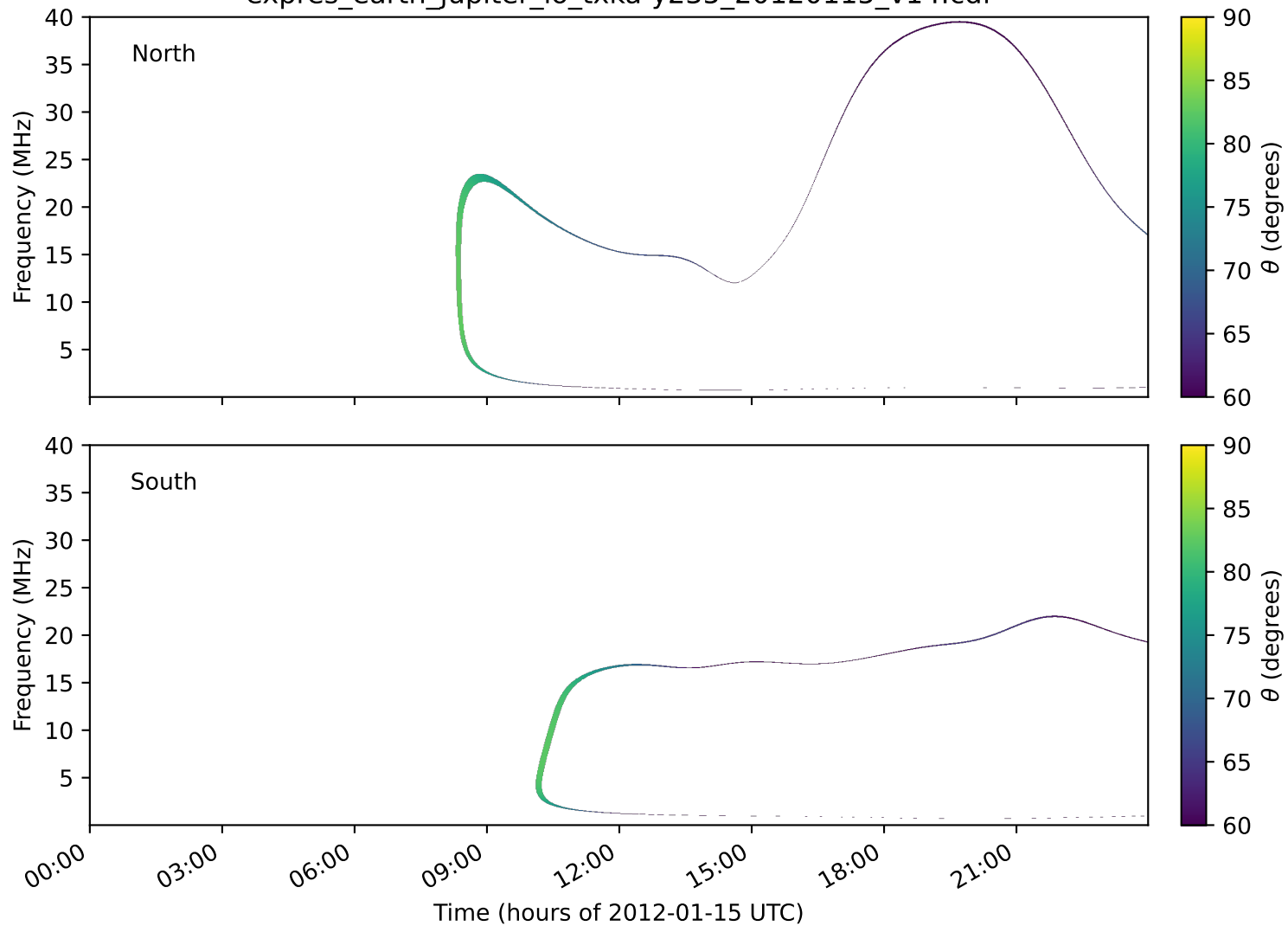
expres_earth_jupiter_io_txka-y235_20120115_v14.cdf
