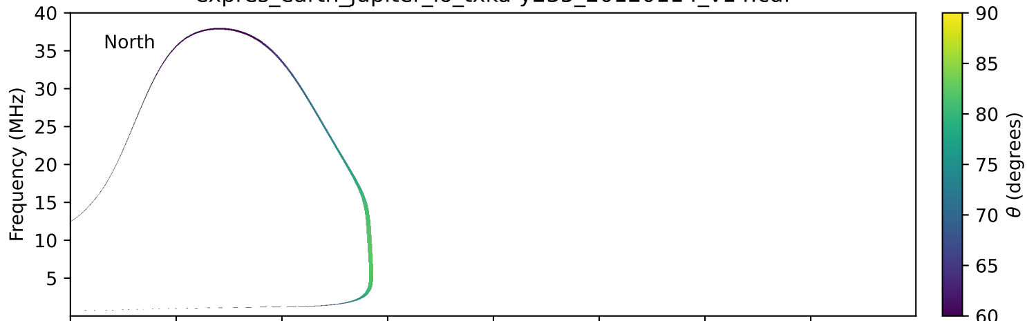
expres_earth_jupiter_io_txka-y235_20120114_v14.cdf
