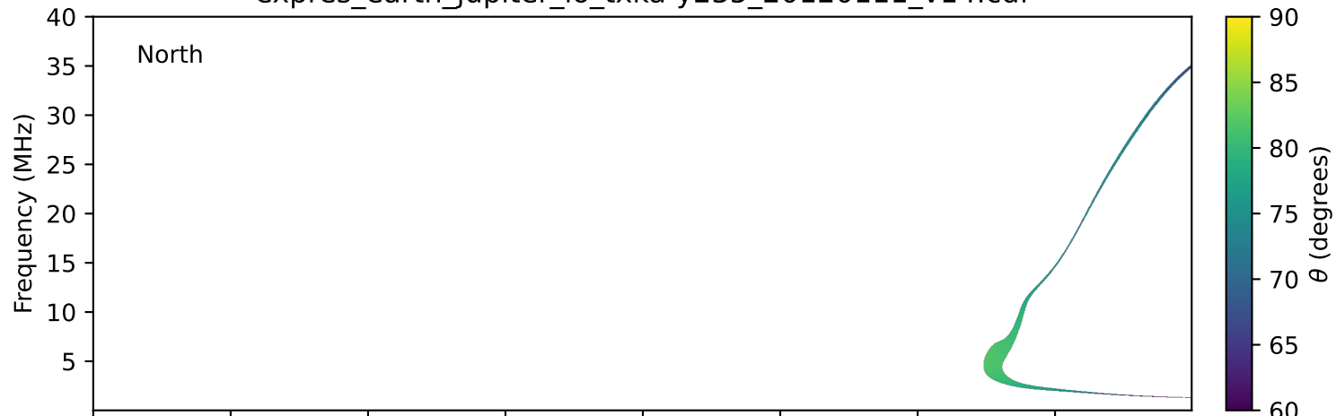
expres_earth_jupiter_io_txka-y235_20120111_v14.cdf
