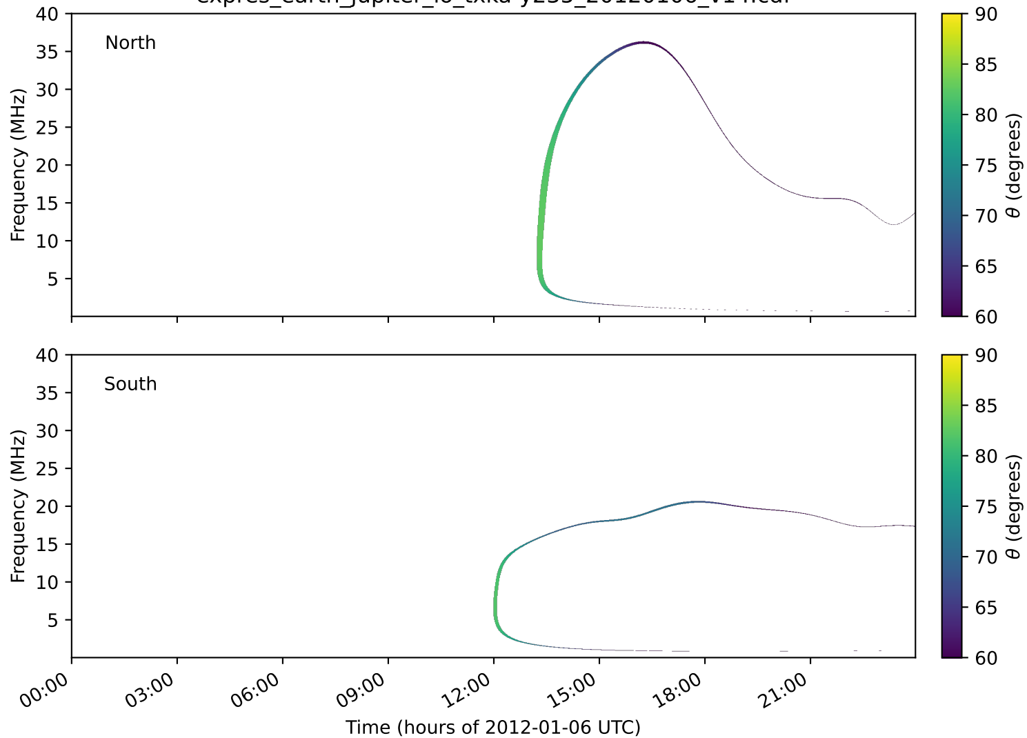
expres_earth_jupiter_io_txka-y235_20120106_v14.cdf
