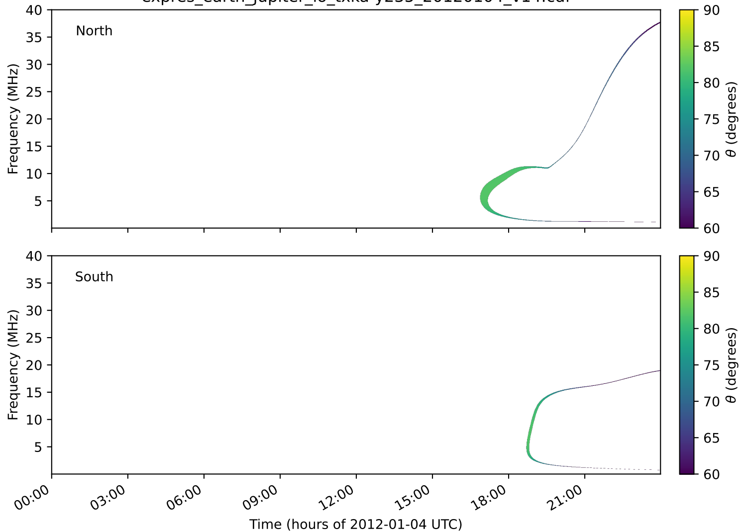
expres_earth_jupiter_io_txka-y235_20120104_v14.cdf
