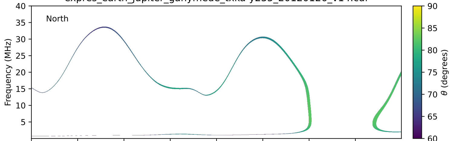
expres_earth_jupiter_ganymede_txka-y235_20120126_v14.cdf
