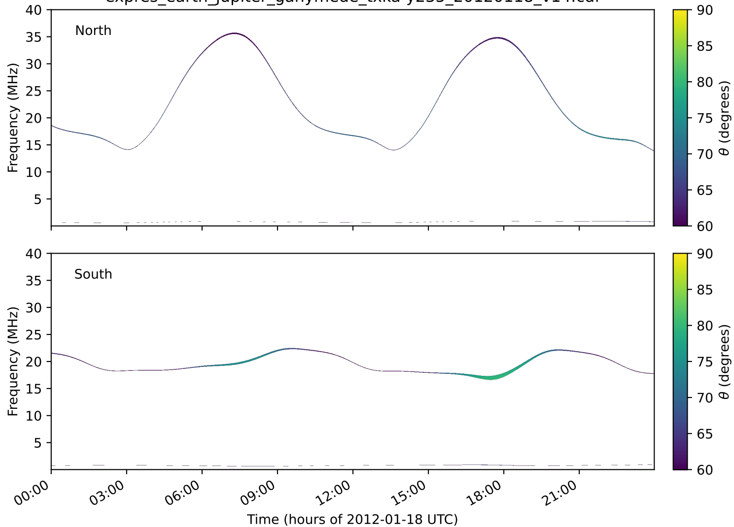
expres_earth_jupiter_ganymede_txka-y235_20120118_v14.cdf
