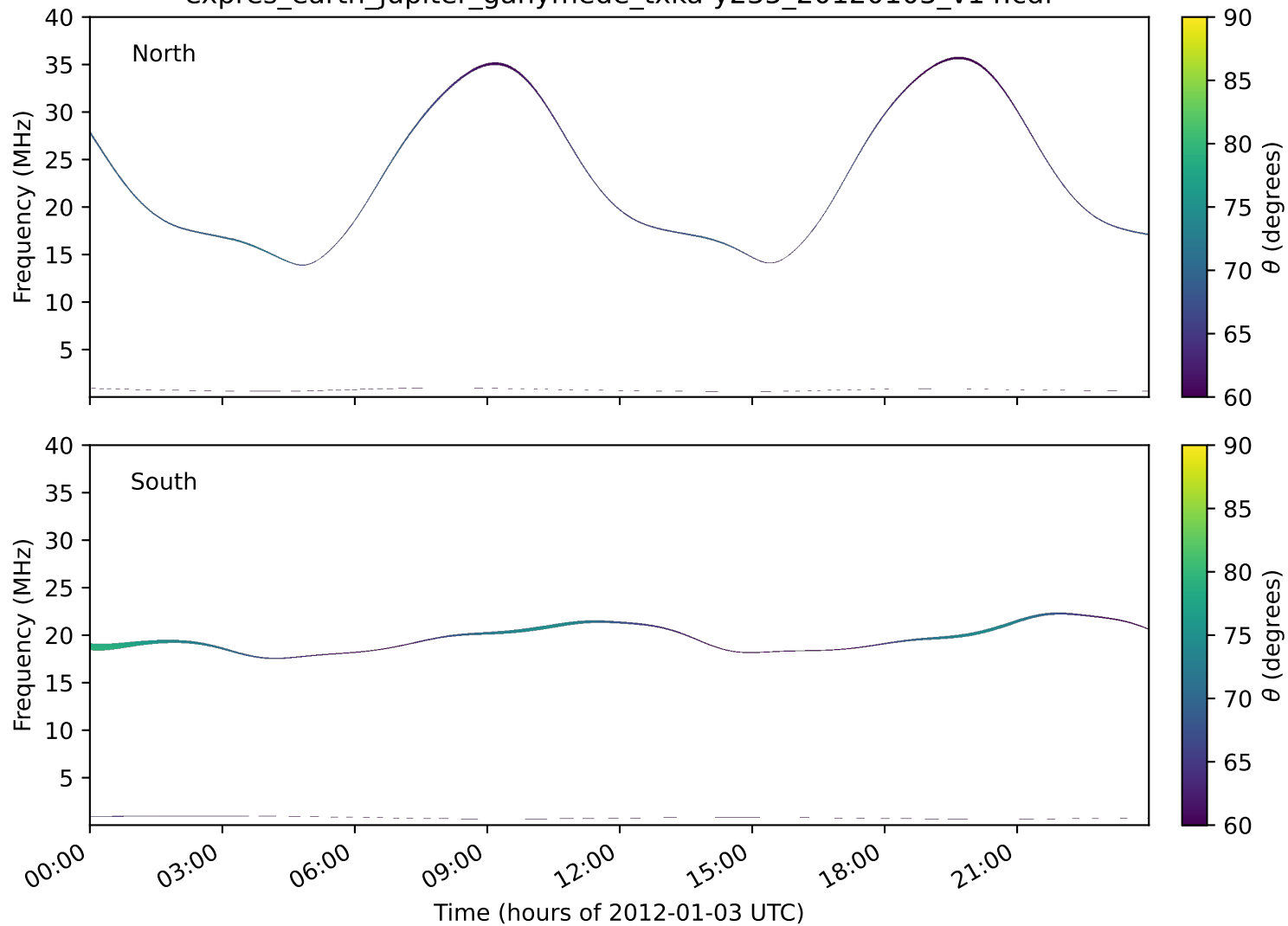
expres_earth_jupiter_ganymede_txka-y235_20120103_v14.cdf
