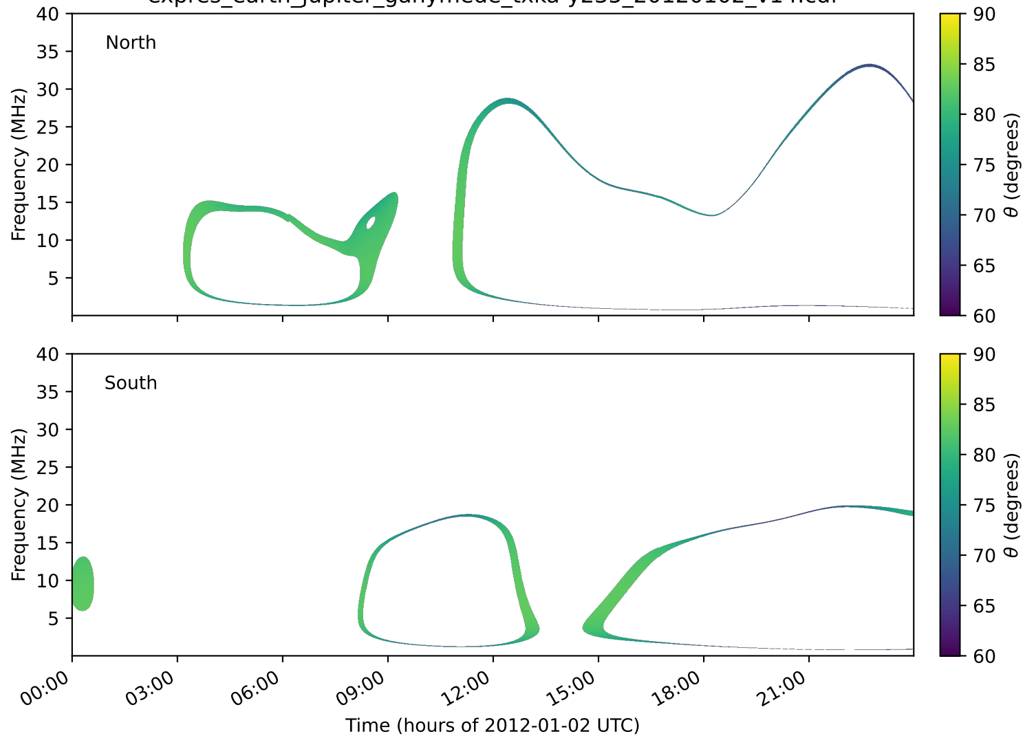
expres_earth_jupiter_ganymede_txka-y235_20120102_v14.cdf
