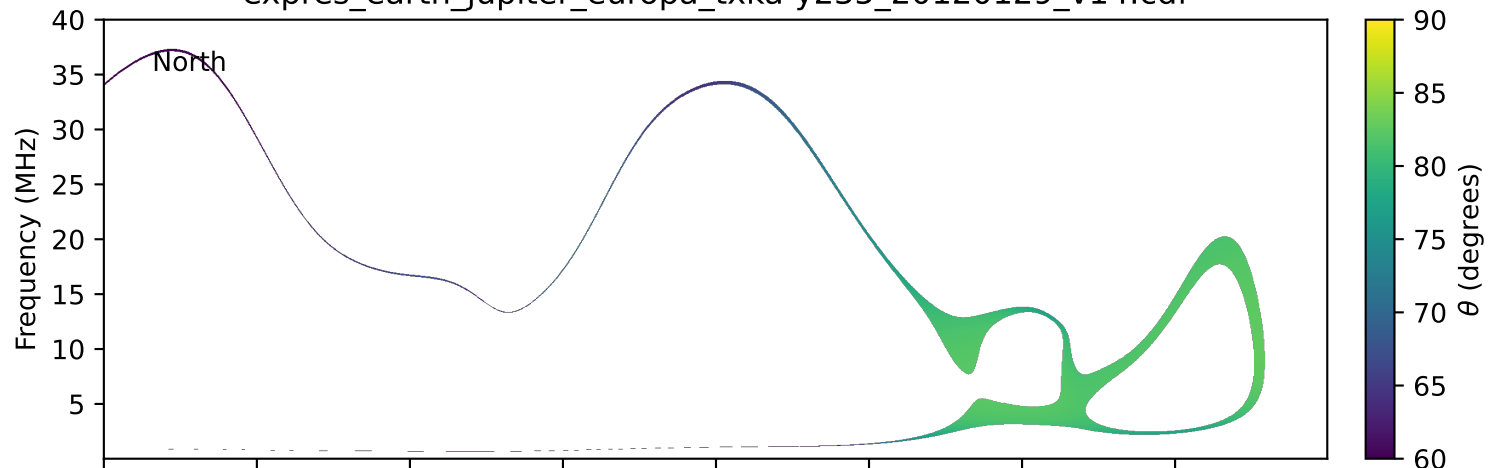
expres_earth_jupiter_europa_txka-y235_20120129_v14.cdf
