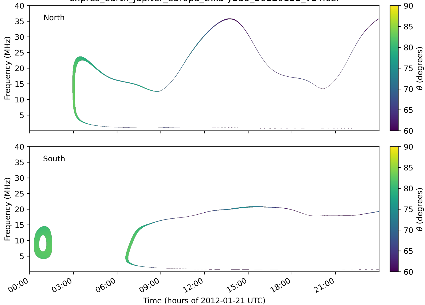
expres_earth_jupiter_europa_txka-y235_20120121_v14.cdf
