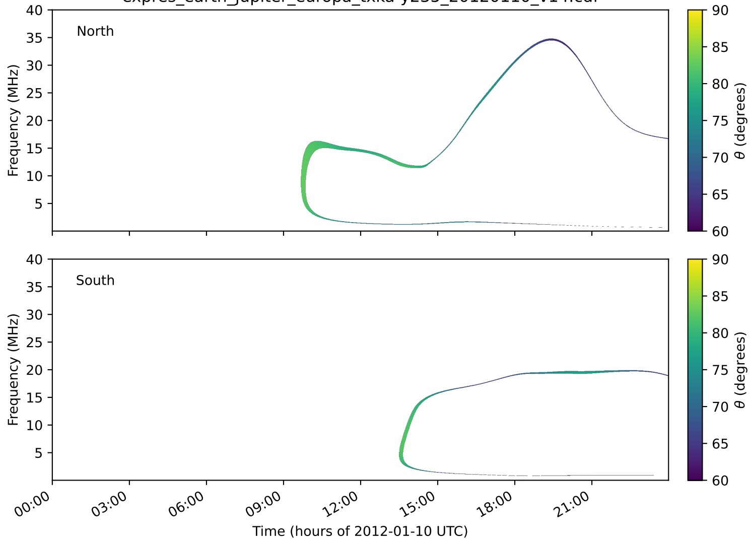
expres_earth_jupiter_europa_txka-y235_20120110_v14.cdf
