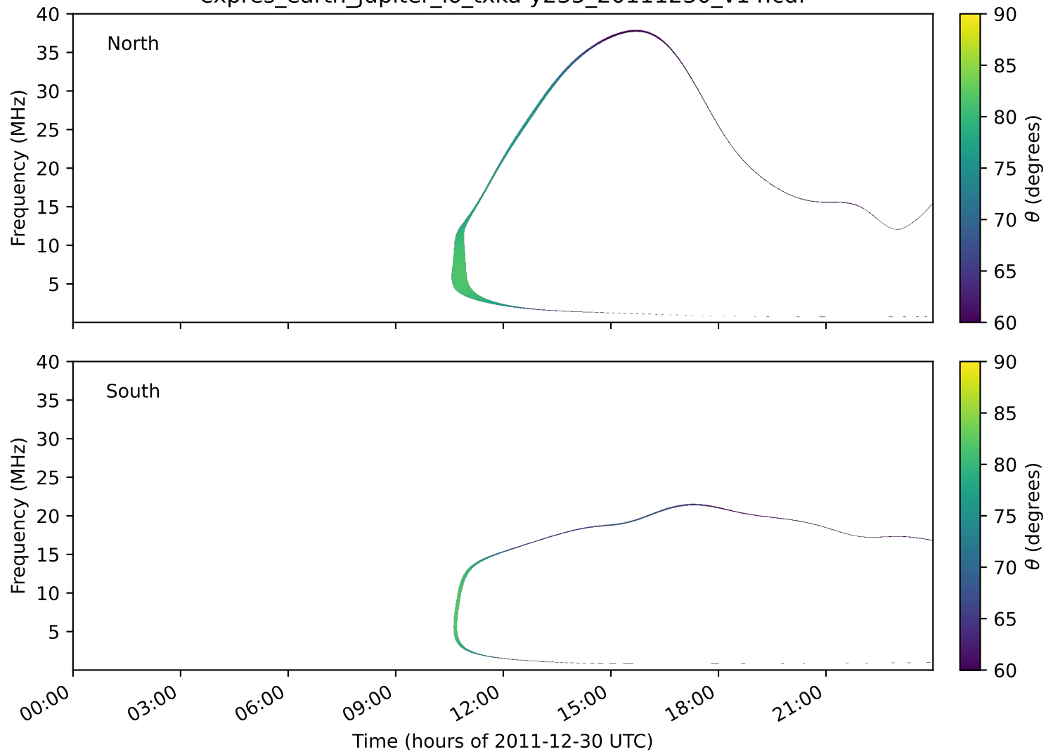
expres_earth_jupiter_io_txka-y235_20111230_v14.cdf
