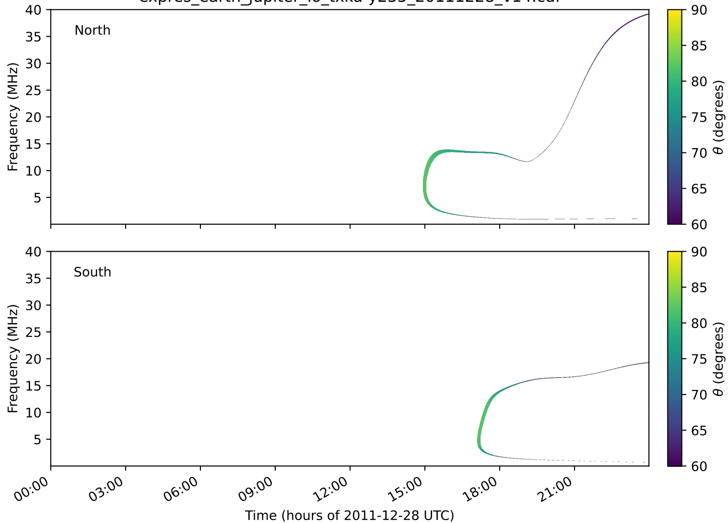
expres_earth_jupiter_io_txka-y235_20111228_v14.cdf
