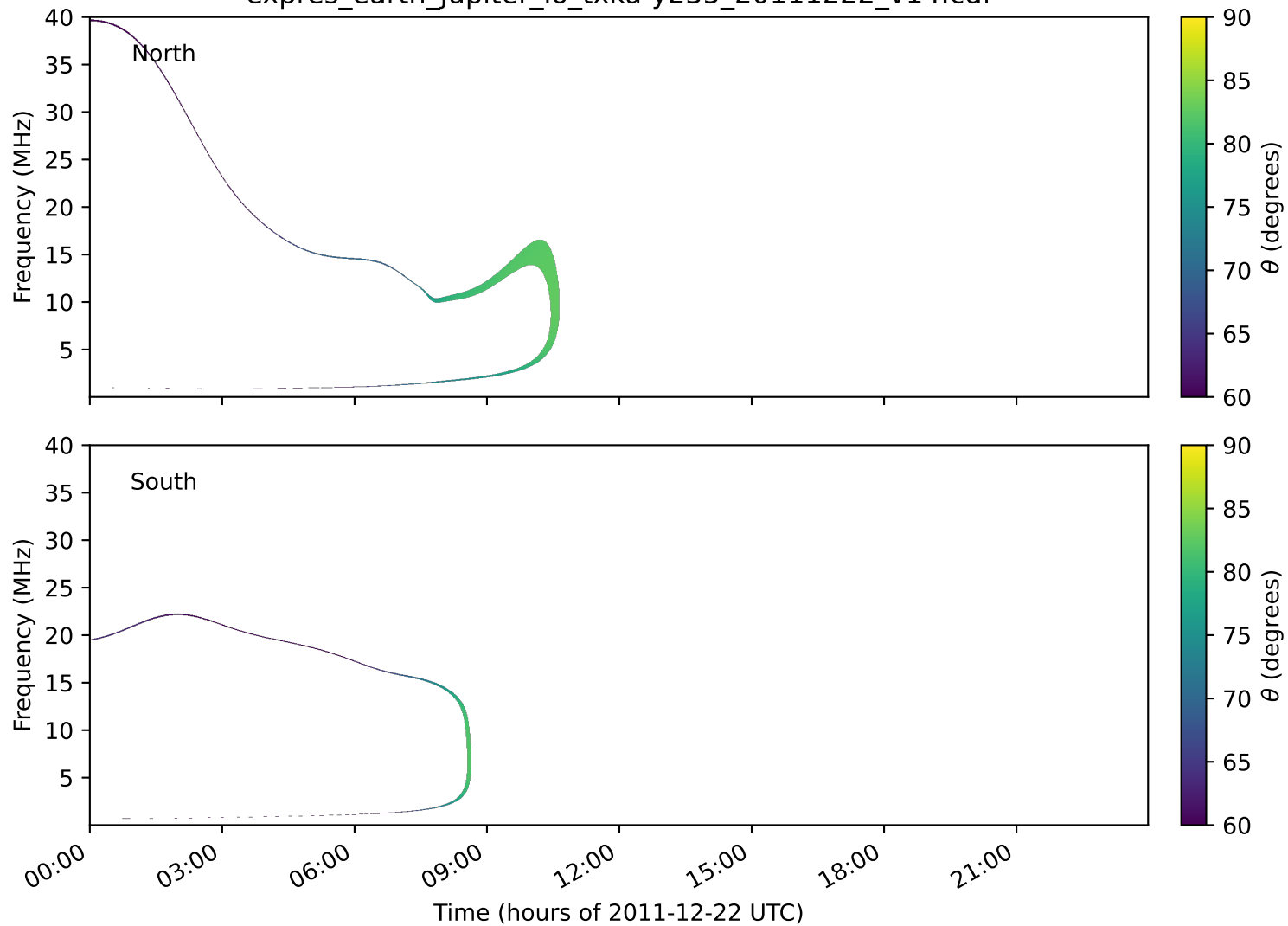
expres_earth_jupiter_io_txka-y235_20111222_v14.cdf
