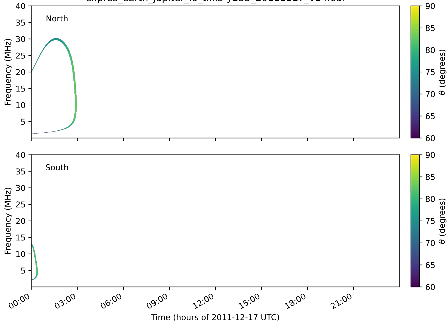
expres_earth_jupiter_io_txka-y235_20111217_v14.cdf
