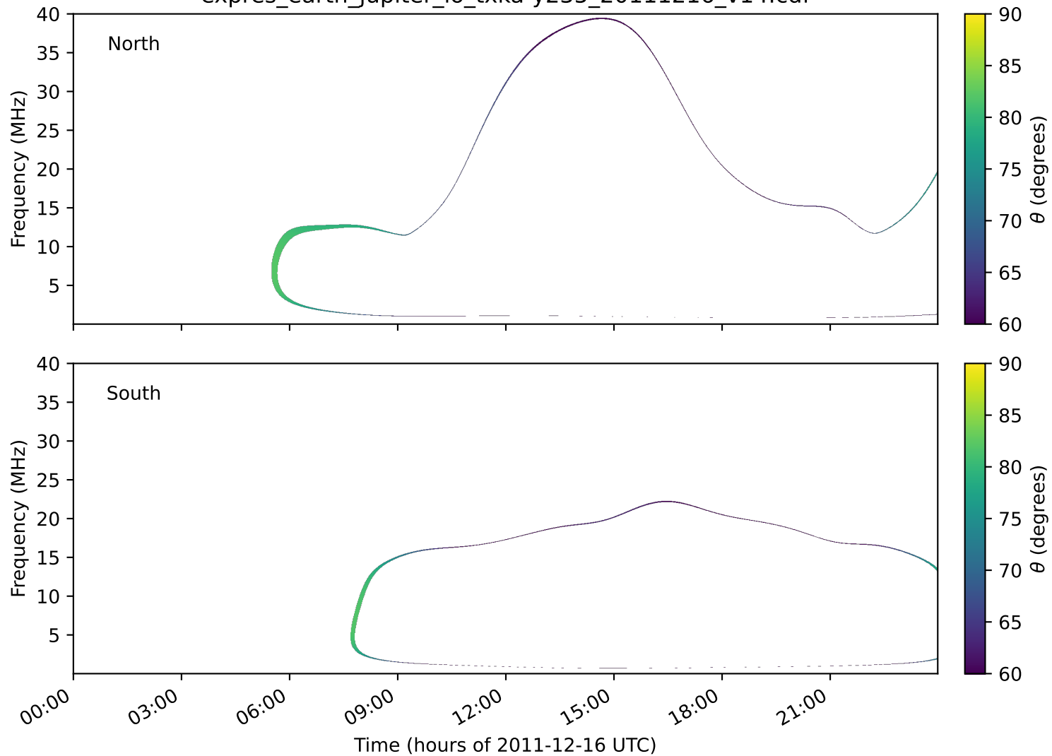
expres_earth_jupiter_io_txka-y235_20111216_v14.cdf
