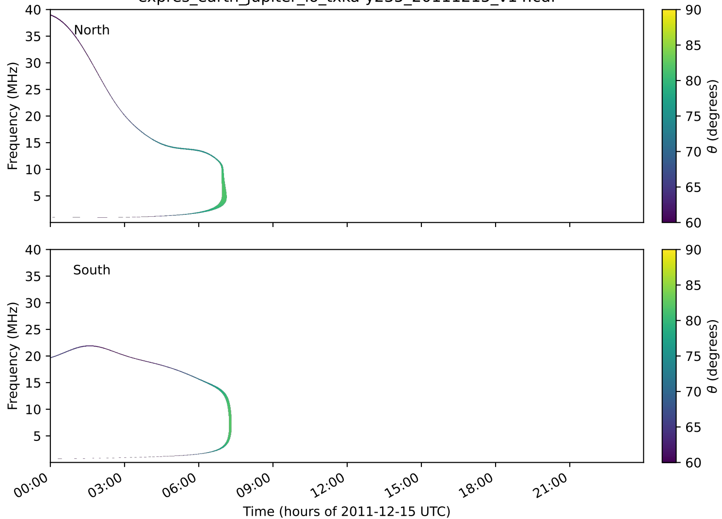
expres_earth_jupiter_io_txka-y235_20111215_v14.cdf
