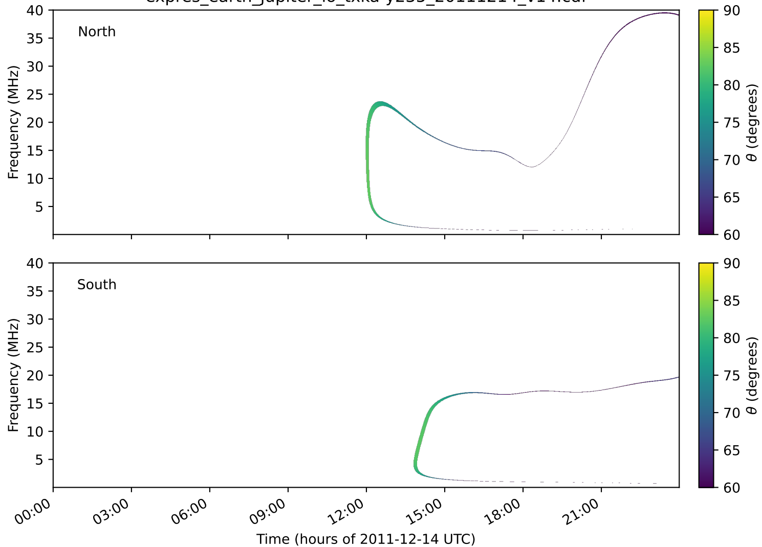
expres_earth_jupiter_io_txka-y235_20111214_v14.cdf
