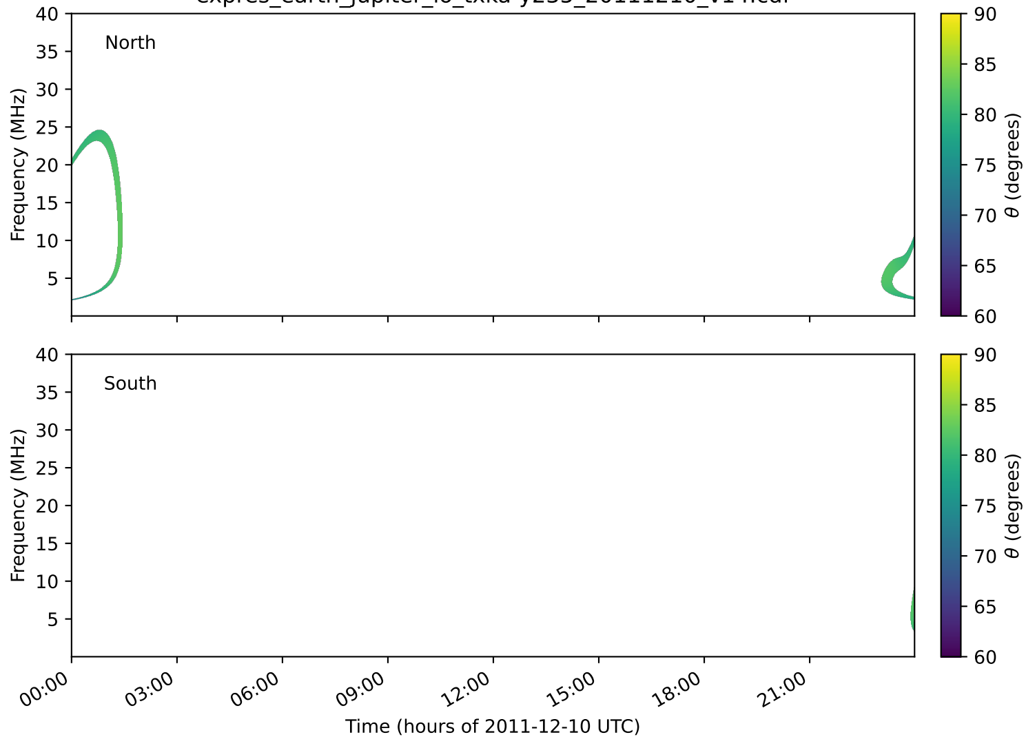
expres_earth_jupiter_io_txka-y235_20111210_v14.cdf
