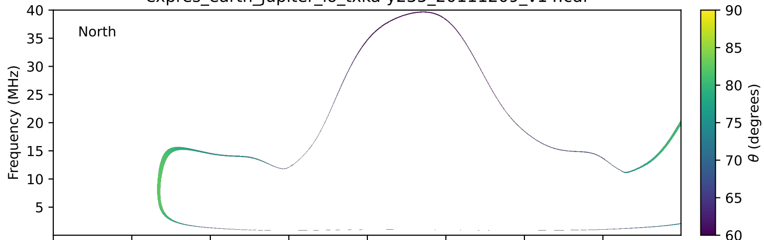
expres_earth_jupiter_io_txka-y235_20111209_v14.cdf
