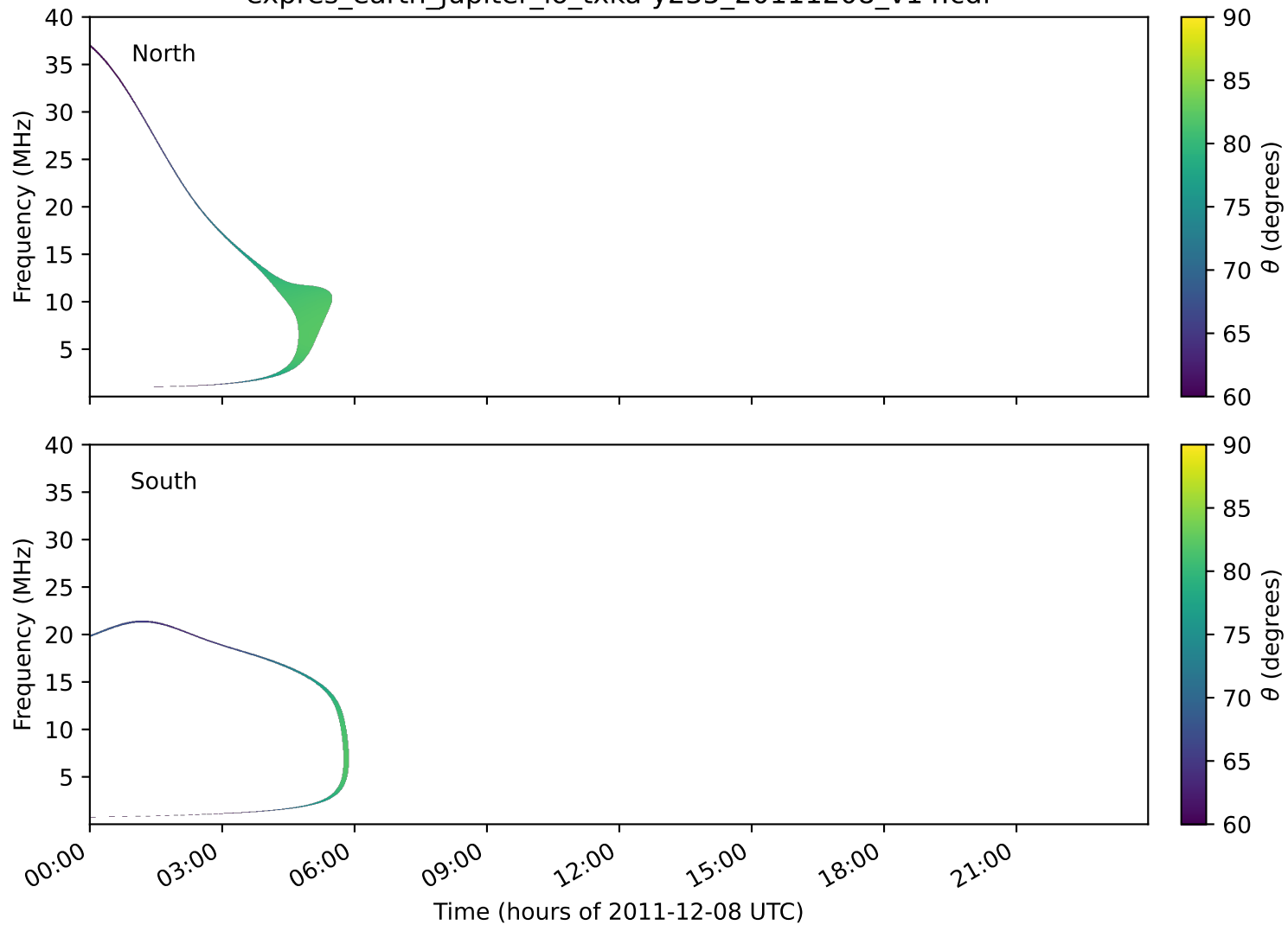
expres_earth_jupiter_io_txka-y235_20111208_v14.cdf
