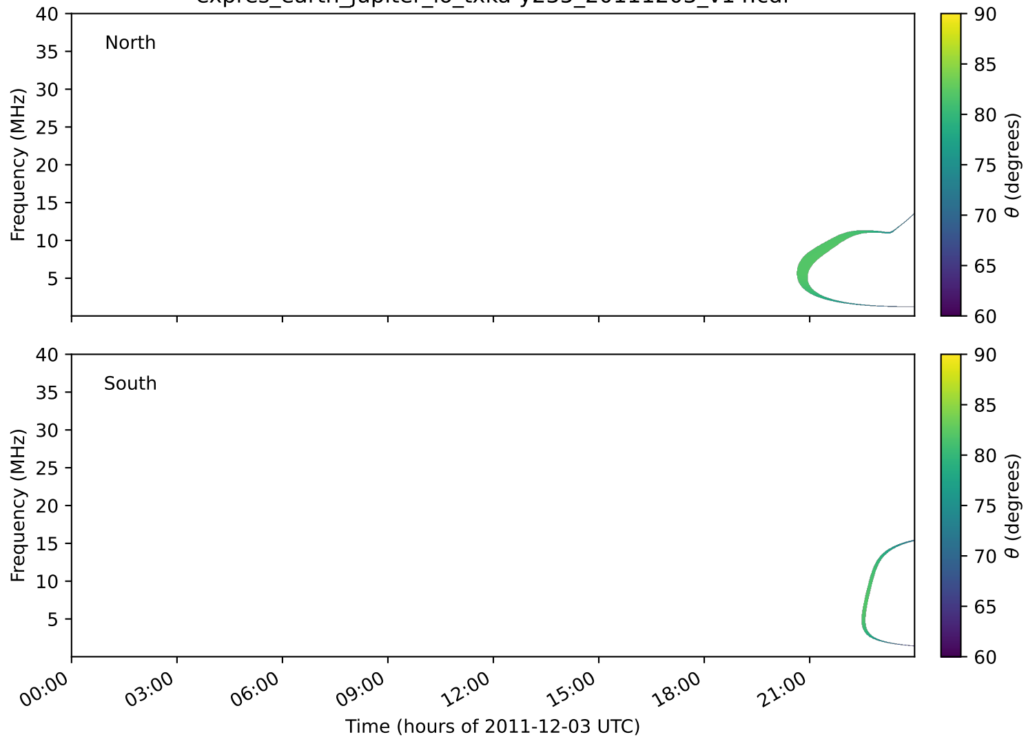
expres_earth_jupiter_io_txka-y235_20111203_v14.cdf
