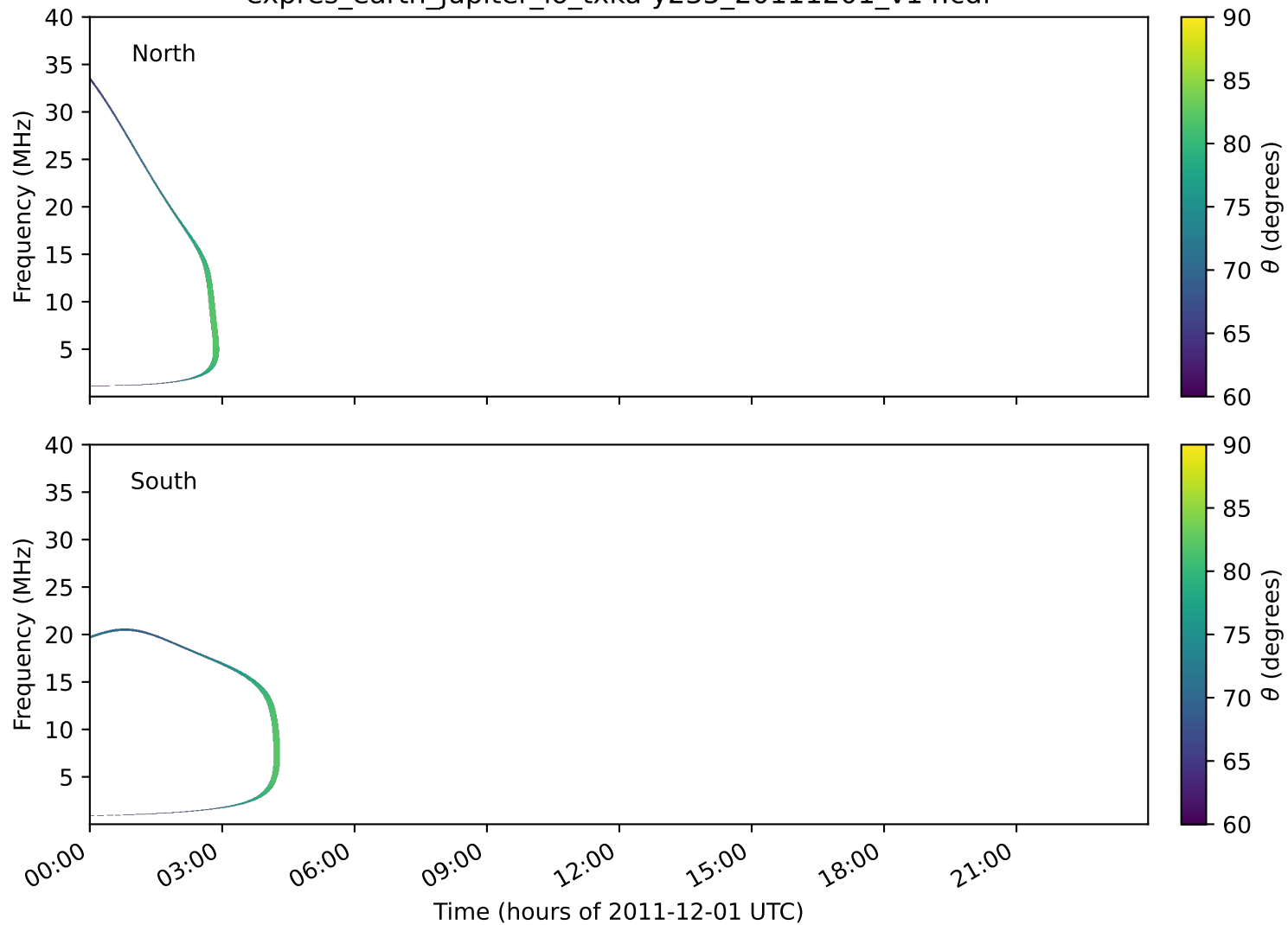
expres_earth_jupiter_io_txka-y235_20111201_v14.cdf
