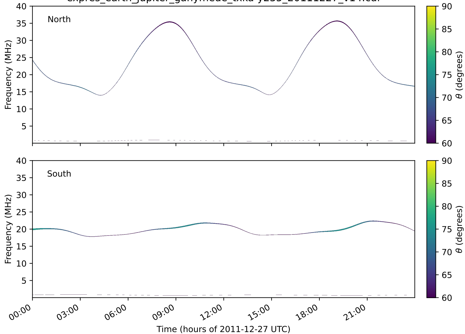
expres_earth_jupiter_ganymede_txka-y235_20111227_v14.cdf
