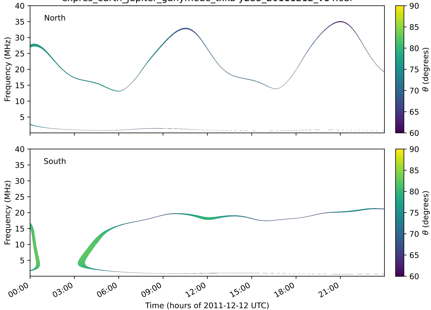
expres_earth_jupiter_ganymede_txka-y235_20111212_v14.cdf
