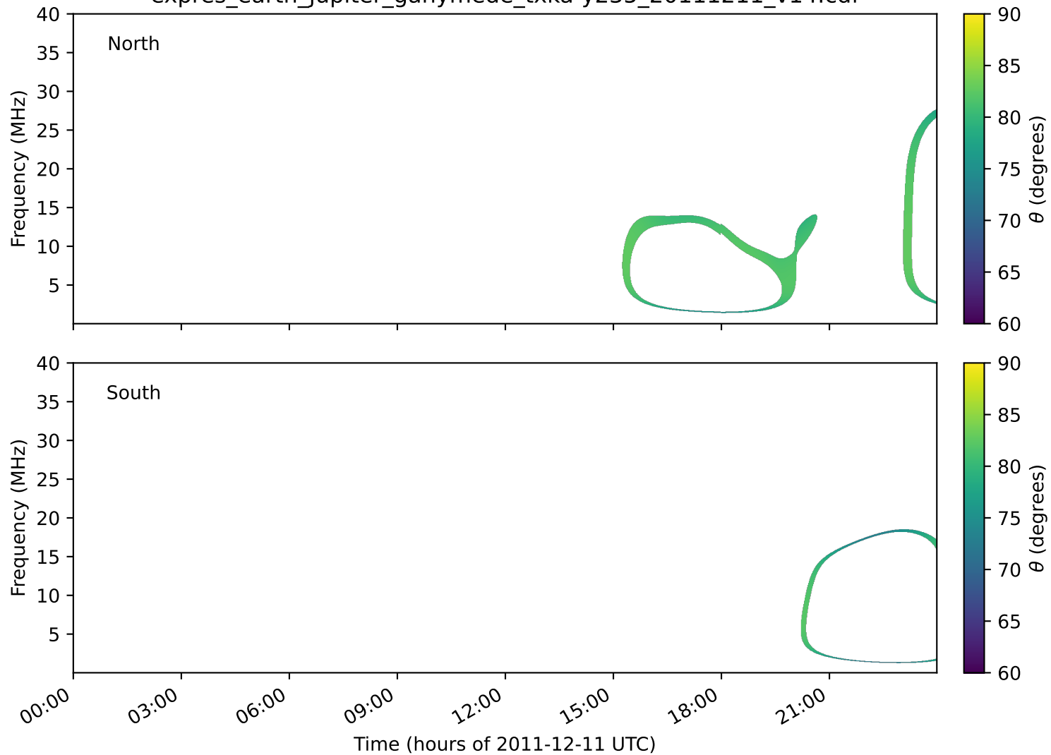
expres_earth_jupiter_ganymede_txka-y235_20111211_v14.cdf
