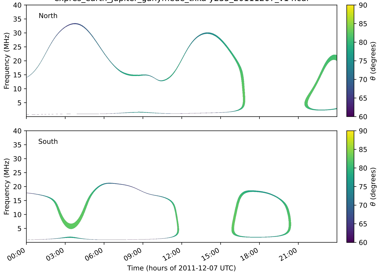
expres_earth_jupiter_ganymede_txka-y235_20111207_v14.cdf
