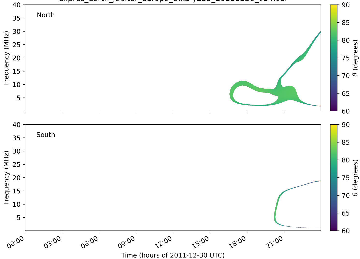
expres_earth_jupiter_europa_txka-y235_20111230_v14.cdf
