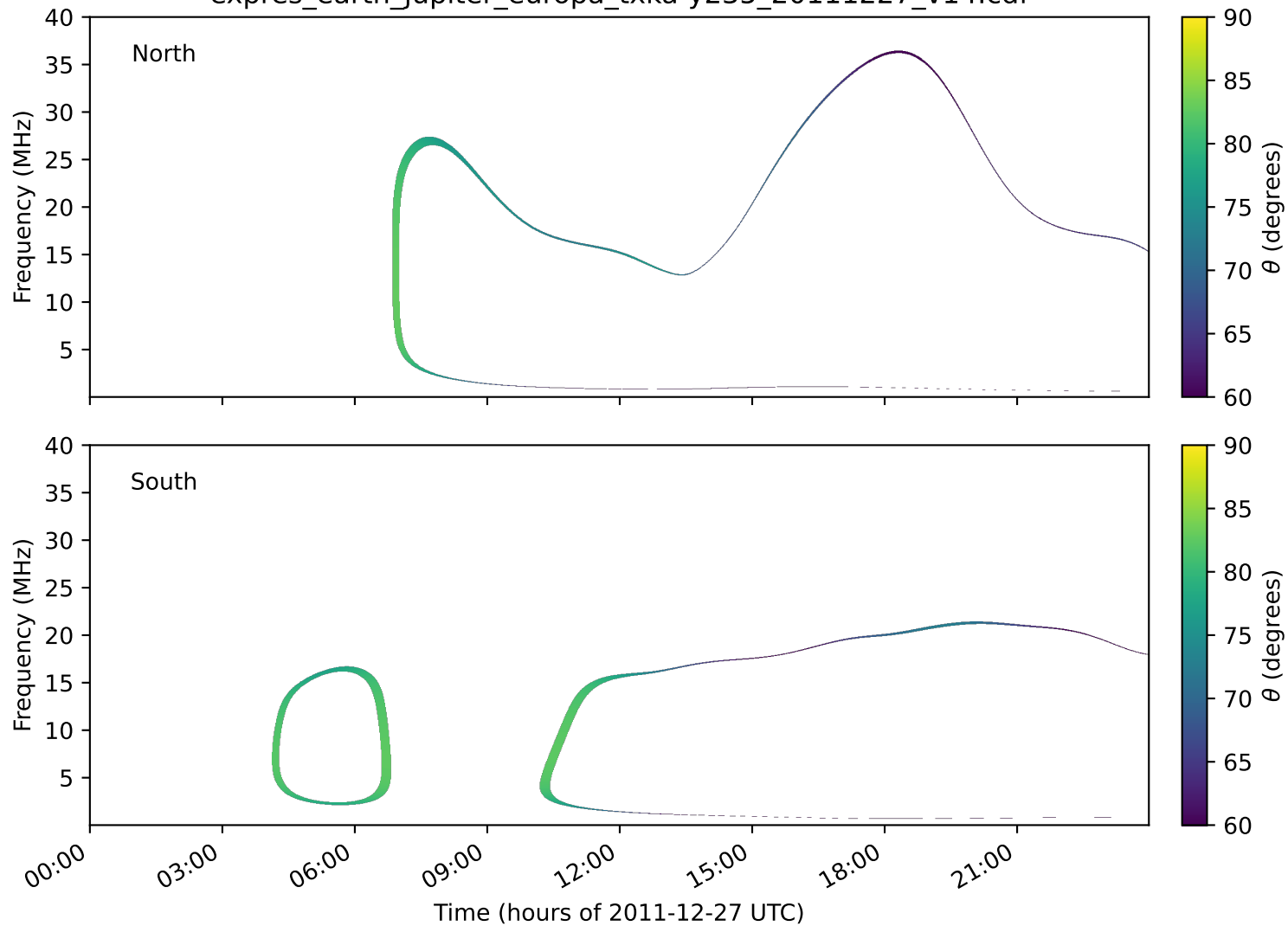
expres_earth_jupiter_europa_txka-y235_20111227_v14.cdf
