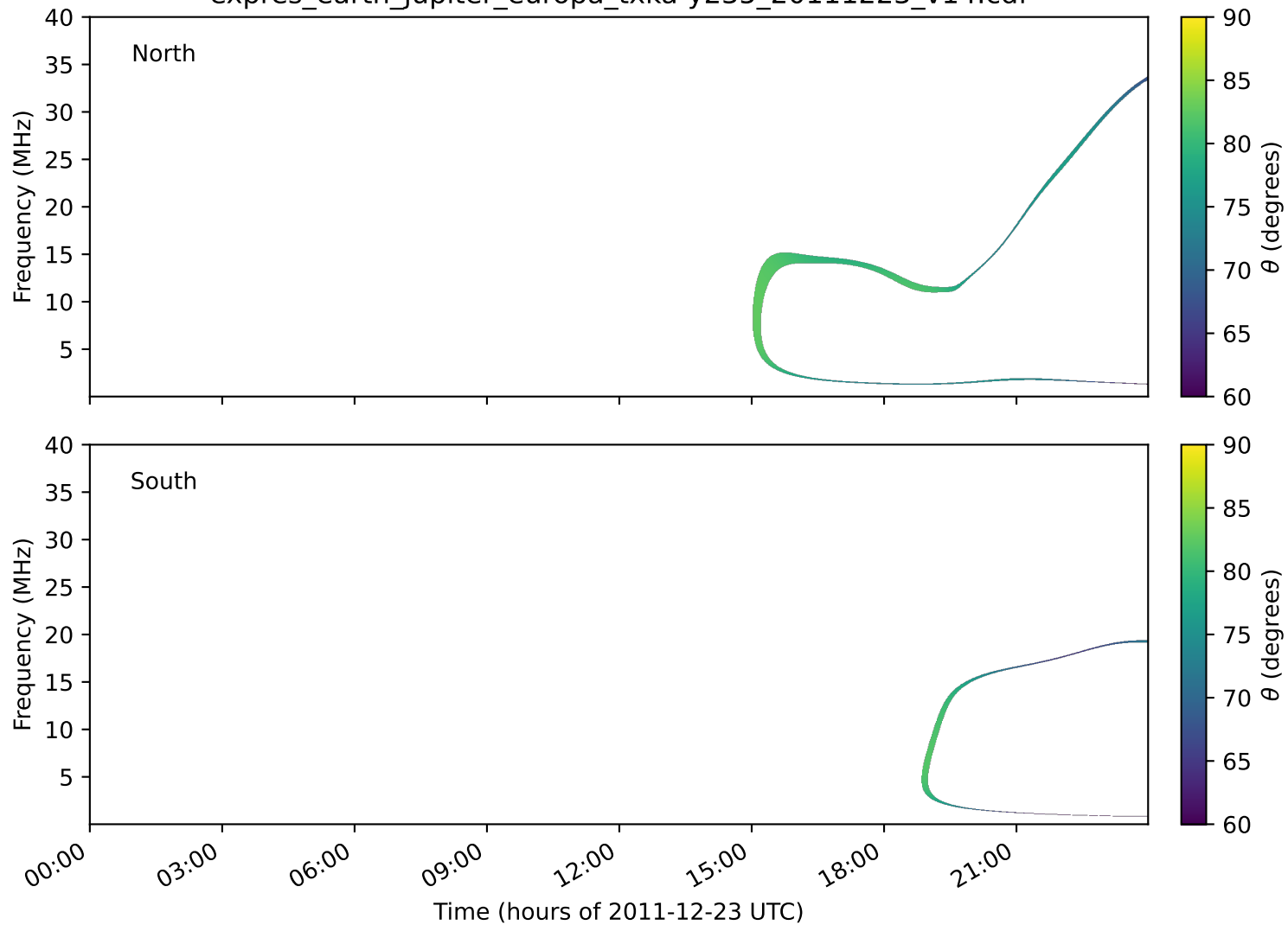
expres_earth_jupiter_europa_txka-y235_20111223_v14.cdf
