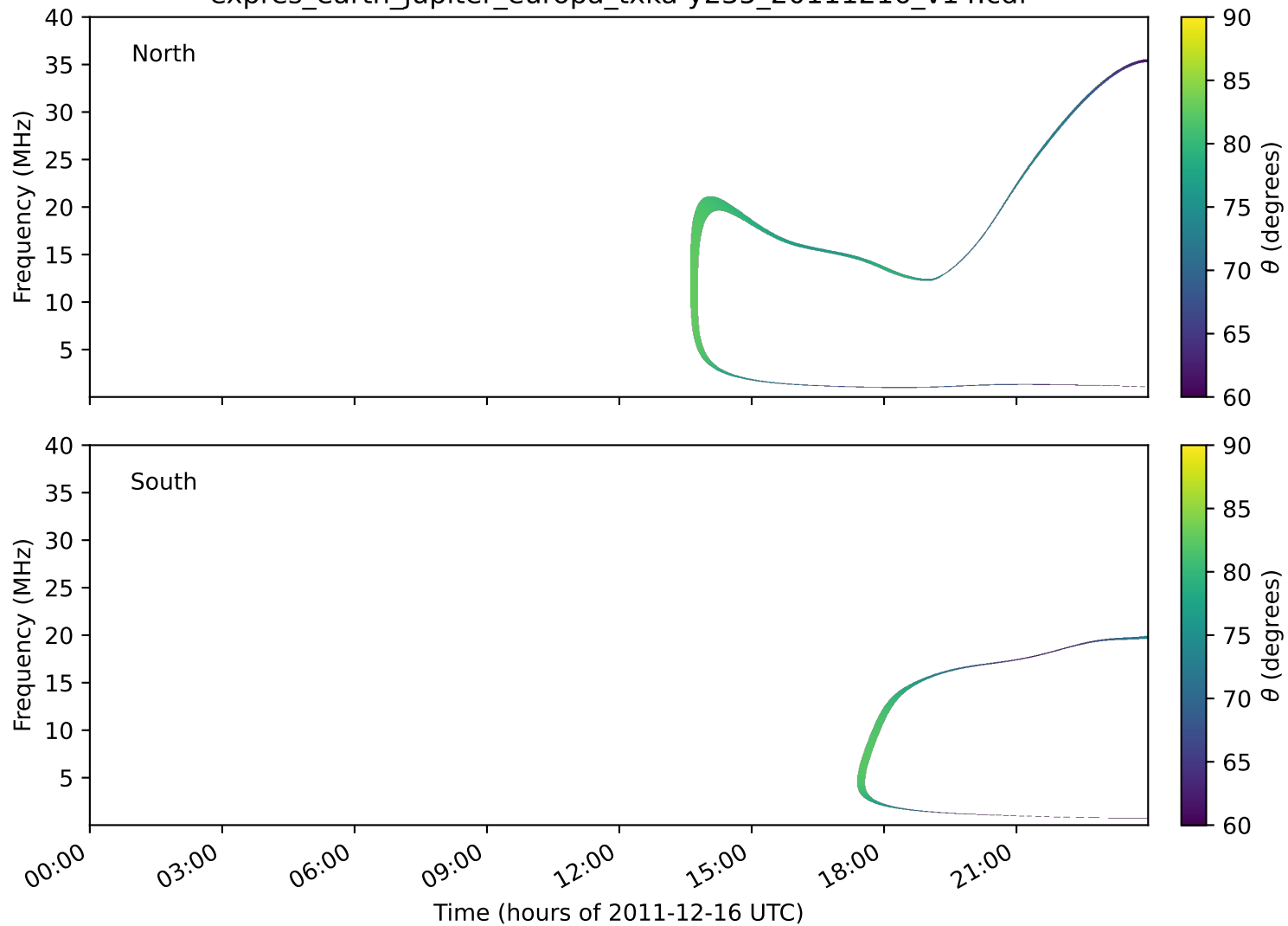
expres_earth_jupiter_europa_txka-y235_20111216_v14.cdf
