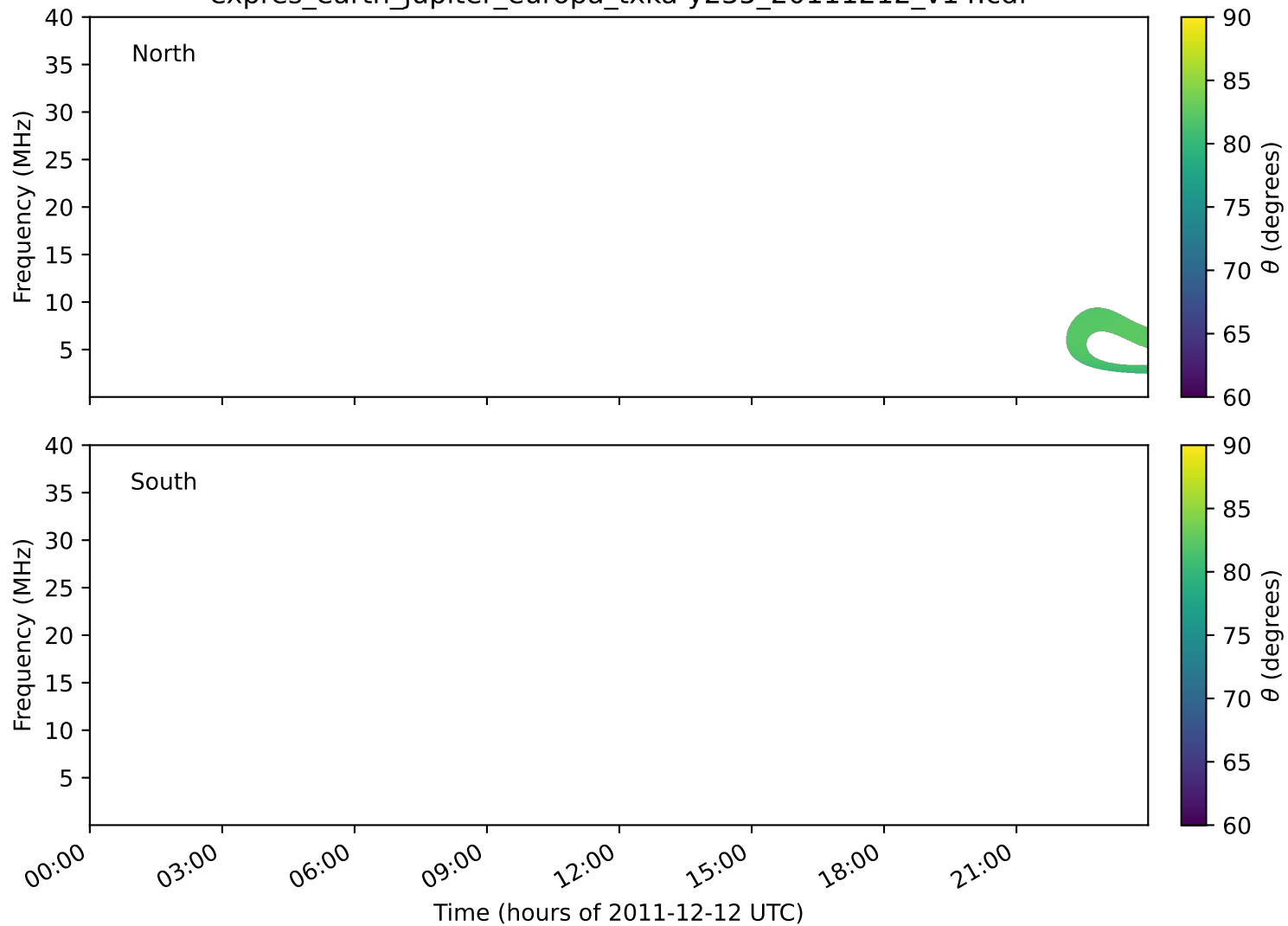
expres_earth_jupiter_europa_txka-y235_20111212_v14.cdf
