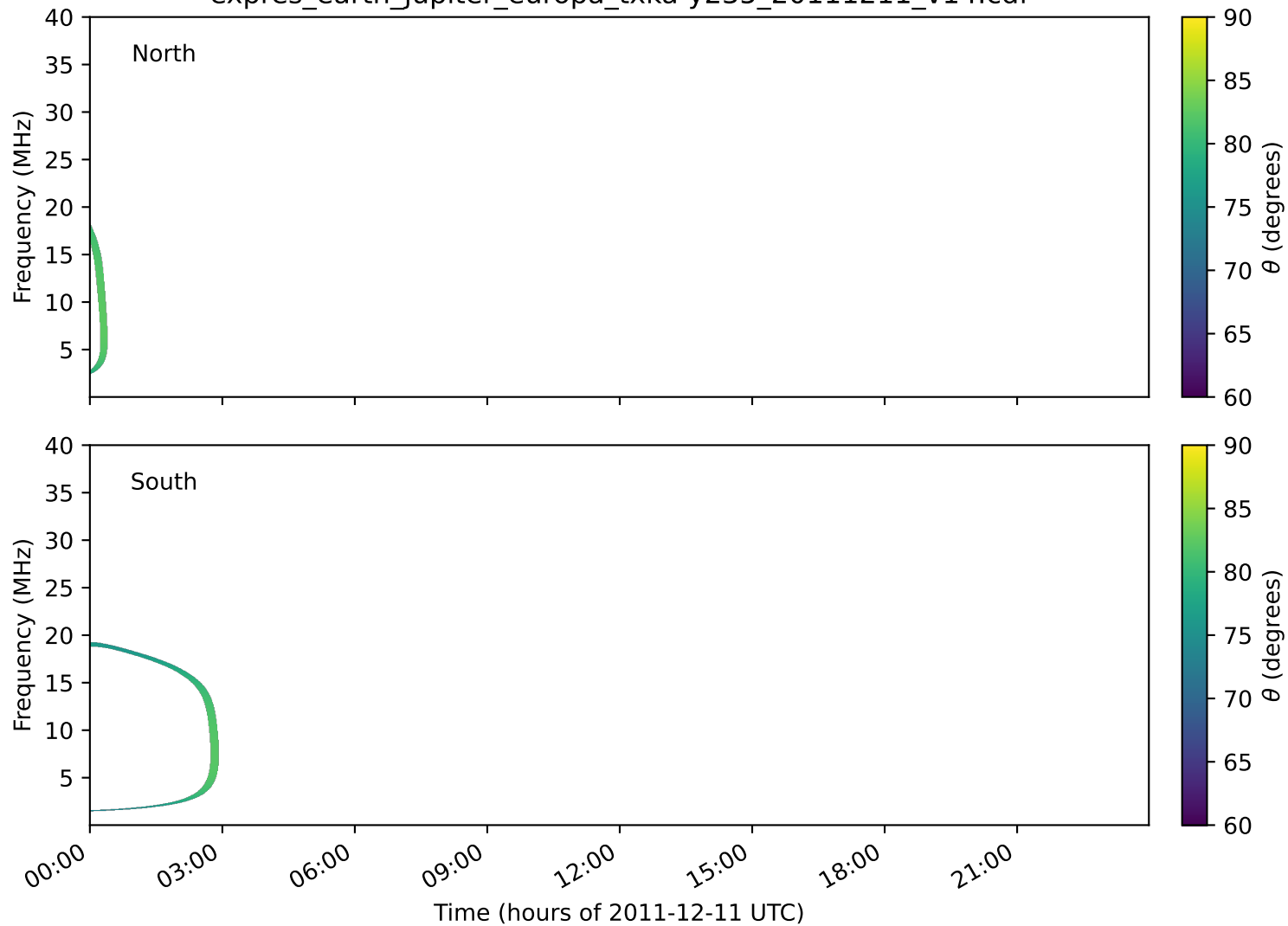
expres_earth_jupiter_europa_txka-y235_20111211_v14.cdf
