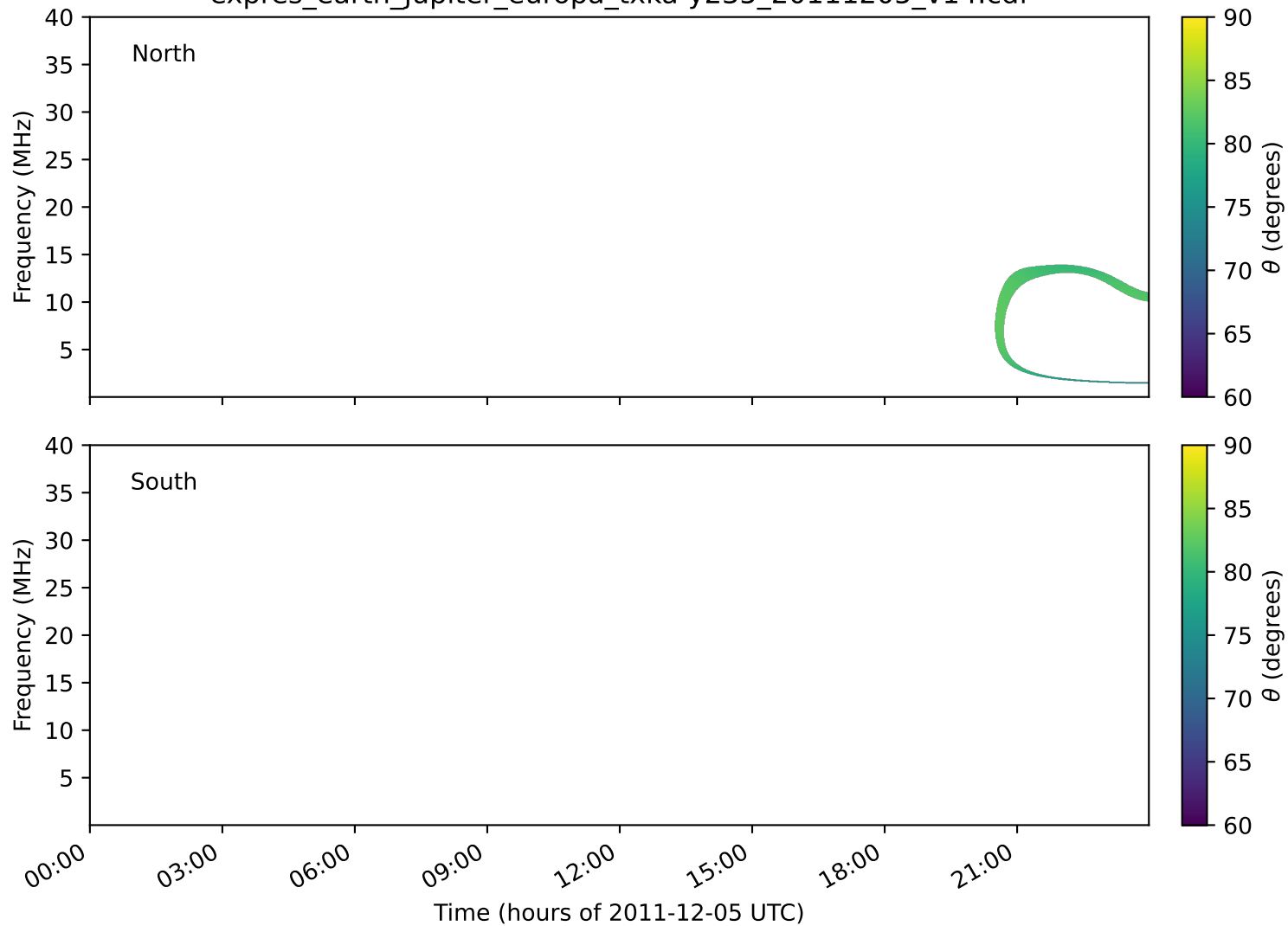
expres_earth_jupiter_europa_txka-y235_20111205_v14.cdf
